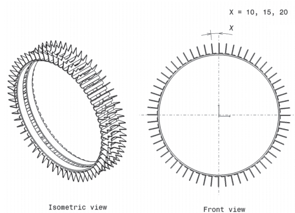
Fig. 5. Dehusking drum with longitudinal profiled blade
