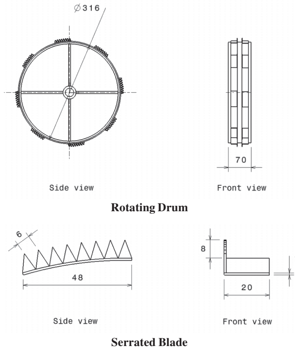
Fig. 4. Dehusking drum with saw tooth circumferential blade
