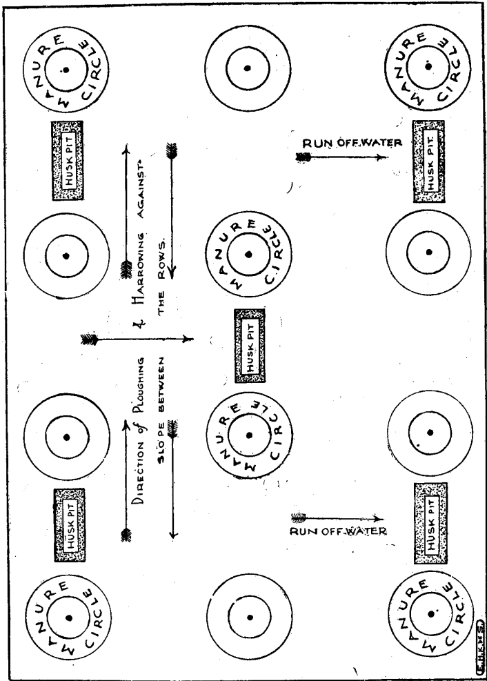
DIAGRAM ARRANGEMENT of HUSK PITS
