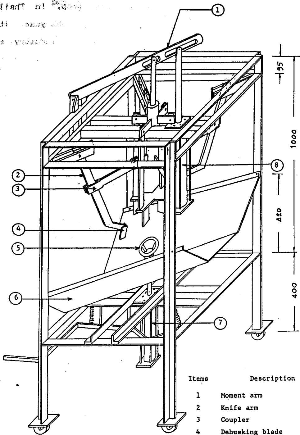
Figure 1. The automatic hydraulic dehusking machine
