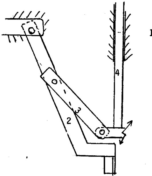
Figure 2. Kinematic diagram of the dehusking mechanism. Link 1 is the frame, link 2 is the knife arm, link 3 is the coupler, link 4 is the slider which is moved in rectilinear translation motion.
