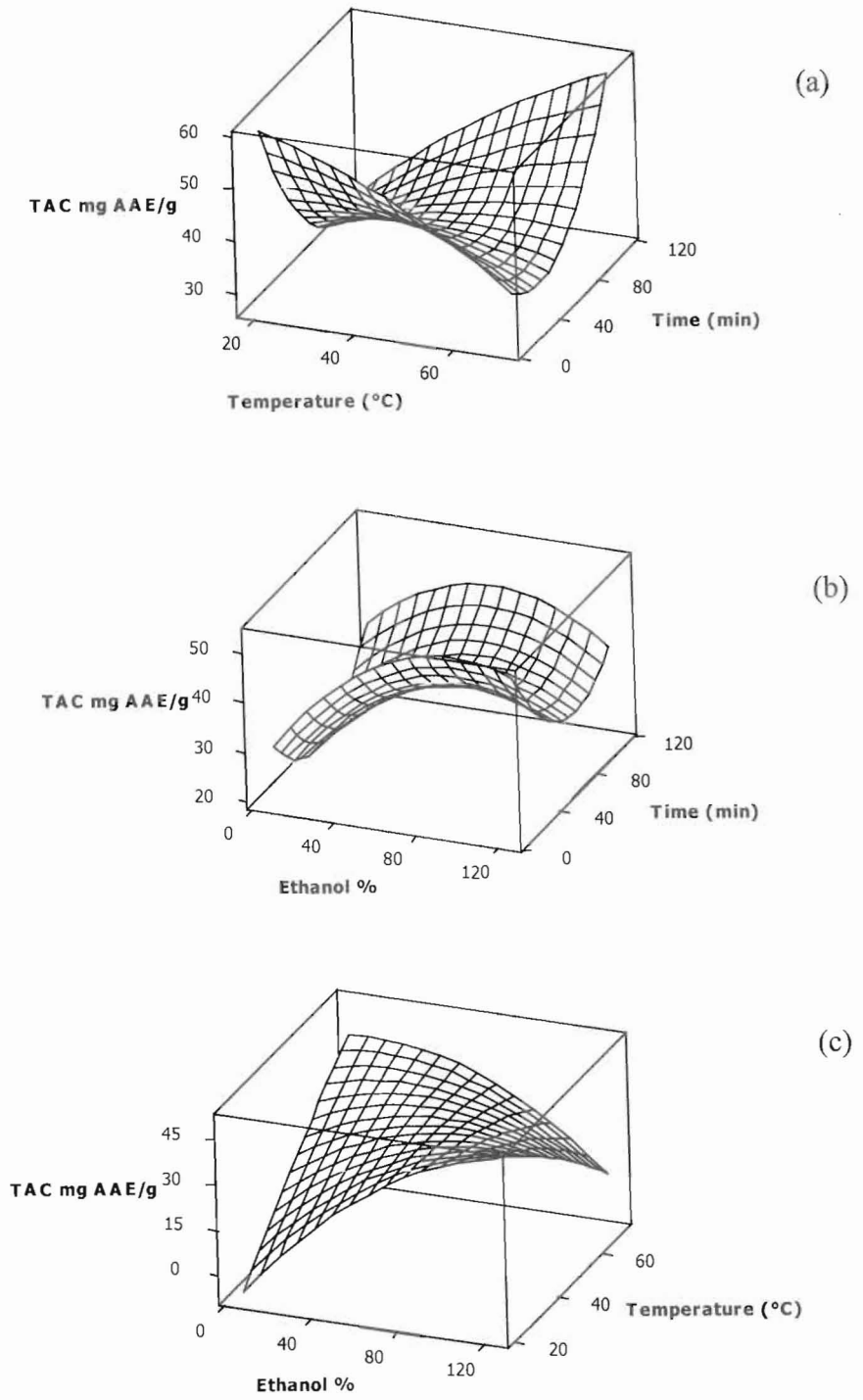
Figure 2. Response surface plots for the total antioxidant capacity (mg AAE/g DW) of the extracts of coconut pairings as a function of ethanol %, extraction temperature and time; ethanol % was kept constant at 65% (a); temperature of extraction was kept constant at 45°C (b) and the time of extraction was kept constant at 60 min (c).
