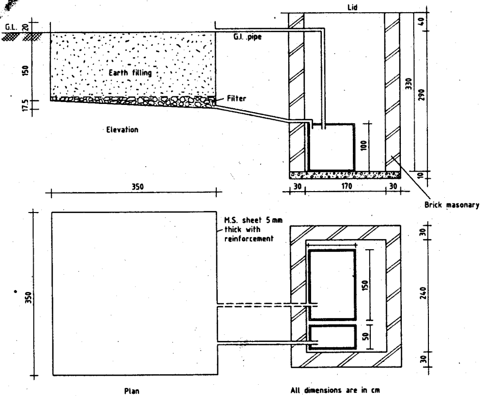
Fig. 1. Lysimeters for ET measurements of coconut palms
