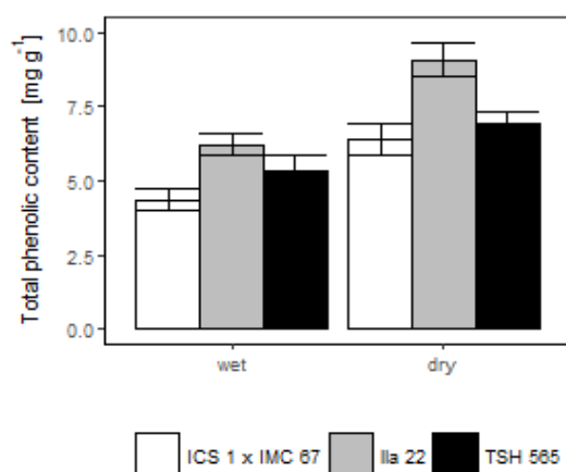
Fig. 3 Total phenolic content in cocoa beans during the wet and the dry season harvest of three cultivars.
