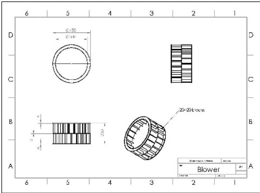
Figure 1. Impeller of blower.
