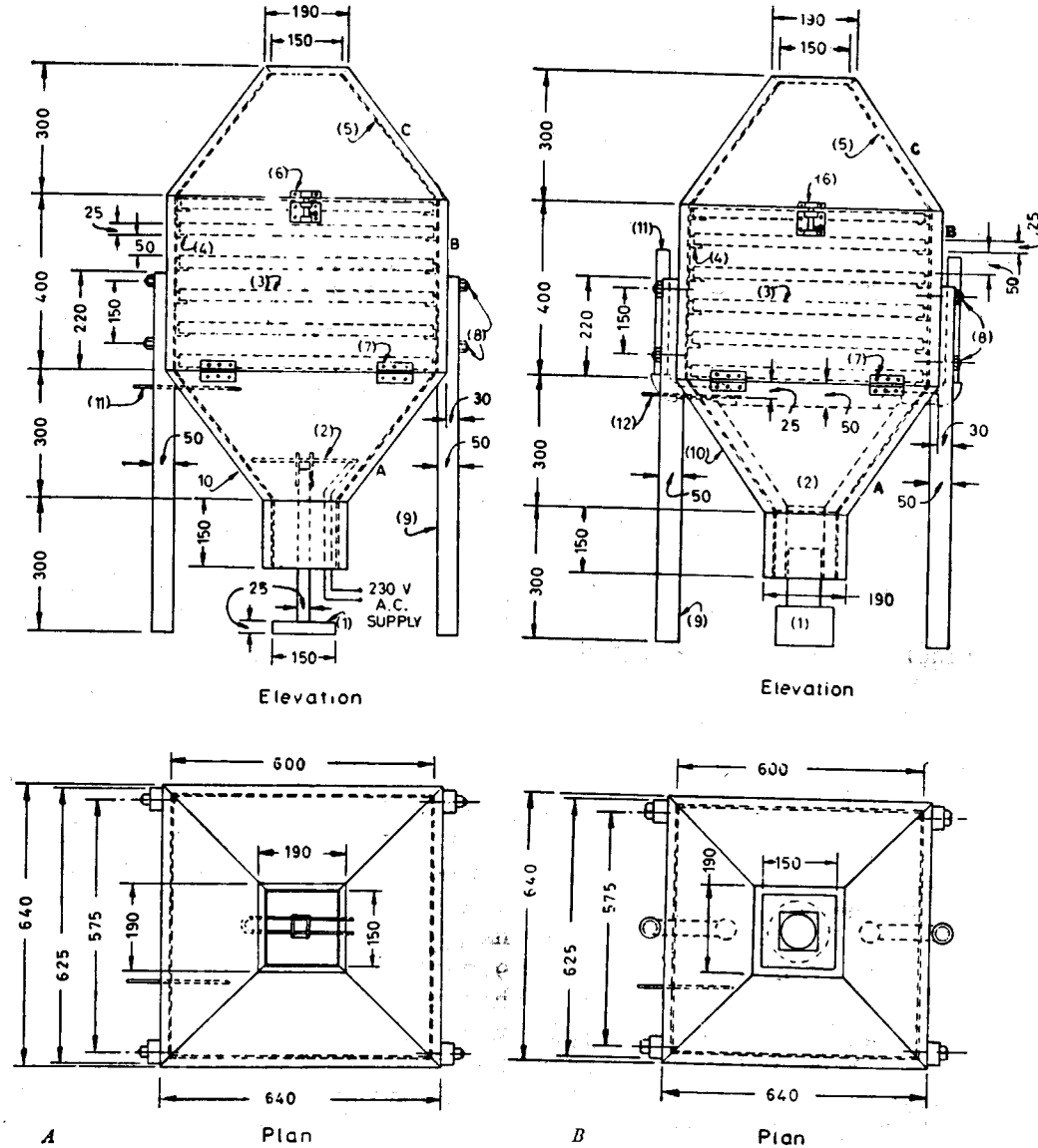
FIG. 1A &amp; B. COCOA BEANS DRIER
