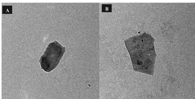
Fig. 4. TEM image of nano-zeolite (A), potassium-impregnated nano-zeolite (B).
