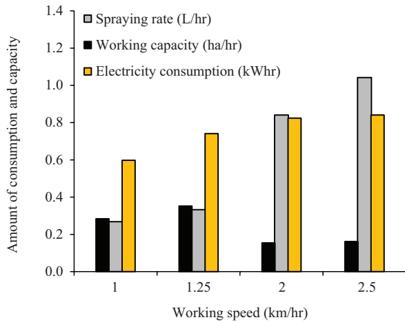
Fig. 6 Field performance of local drone with remote controlled sprayer arm
