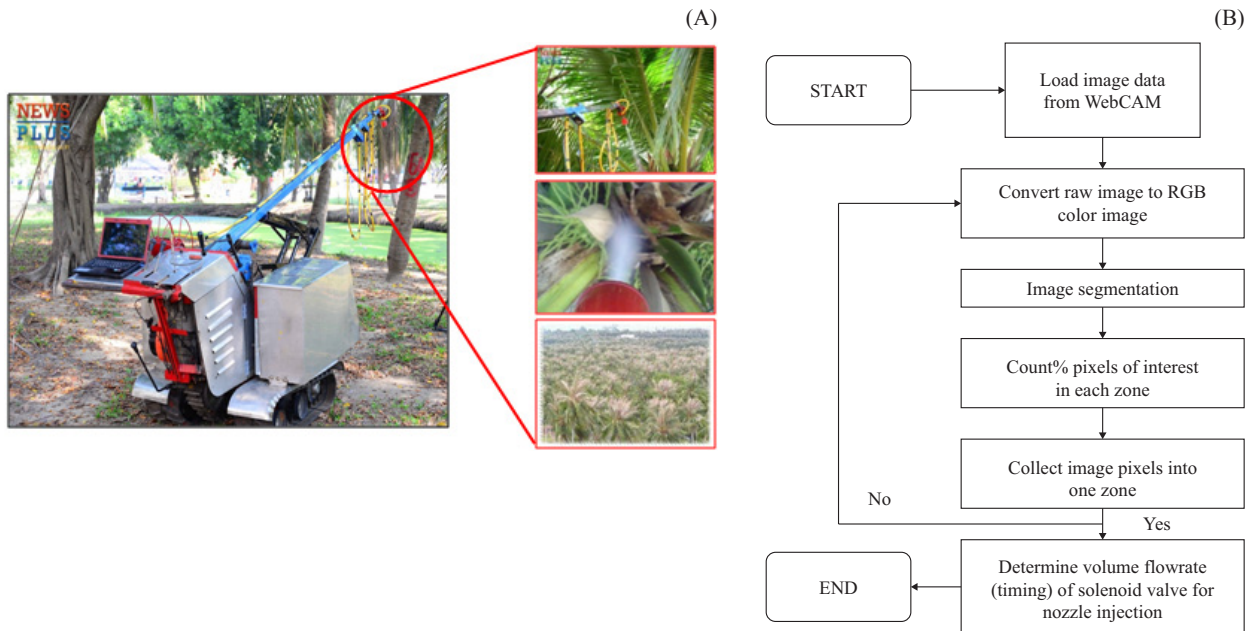
Fig. 3 Design and fabrication of a hardware and a variable rate (VRT) sprayer
