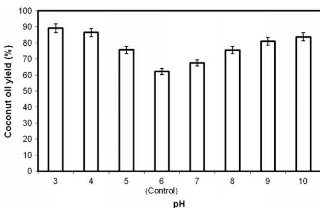
Fig. 2. Effect of pH on the stability of coconut milk emulsion quantified by oil yield.
