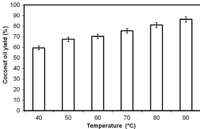
Fig. 1. Effect of thermal treatment on the stability of coconut milk emulsion quantified by oil yield.
