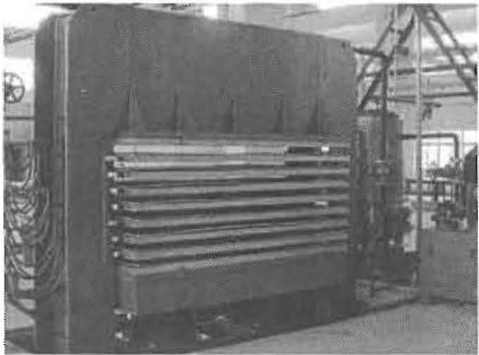
(a) Hydraulic hot press
