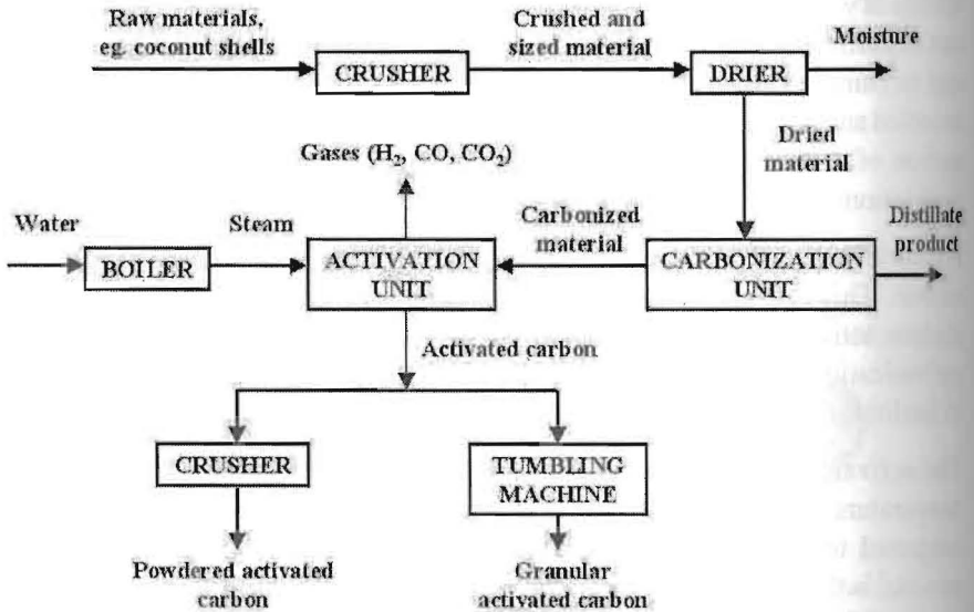
Fig. 6: Process flow chart for production of activated carbon from coconut shell
